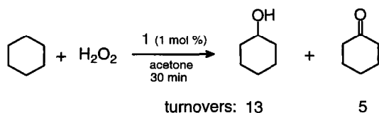
Scheme 3. Catalytic oxidation of cyclohexane with H 2 O 2 using 1 as a catalyst.
