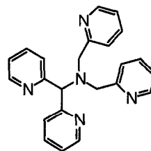
Fig. 2. The new pentadentate ligand, N4Py.
